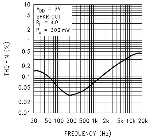
THD+N vs Frequency LM4856LQ
